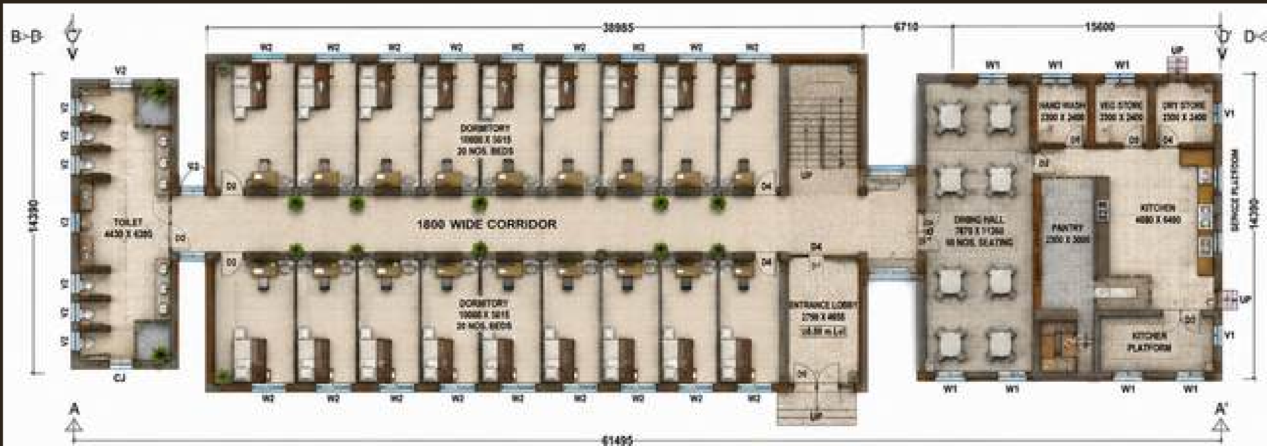
GROUND FLOOR PLAN 620.00 SQMTS
